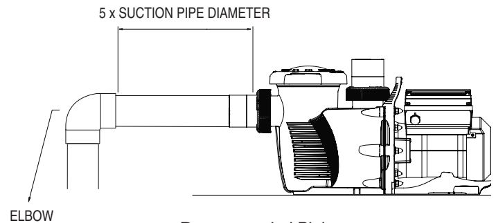
Recommended Piping
