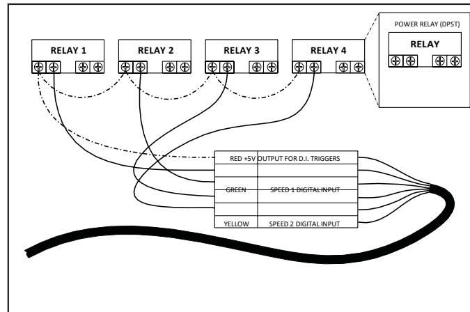
Figure 10: External Control Kit Wiring Diagram
