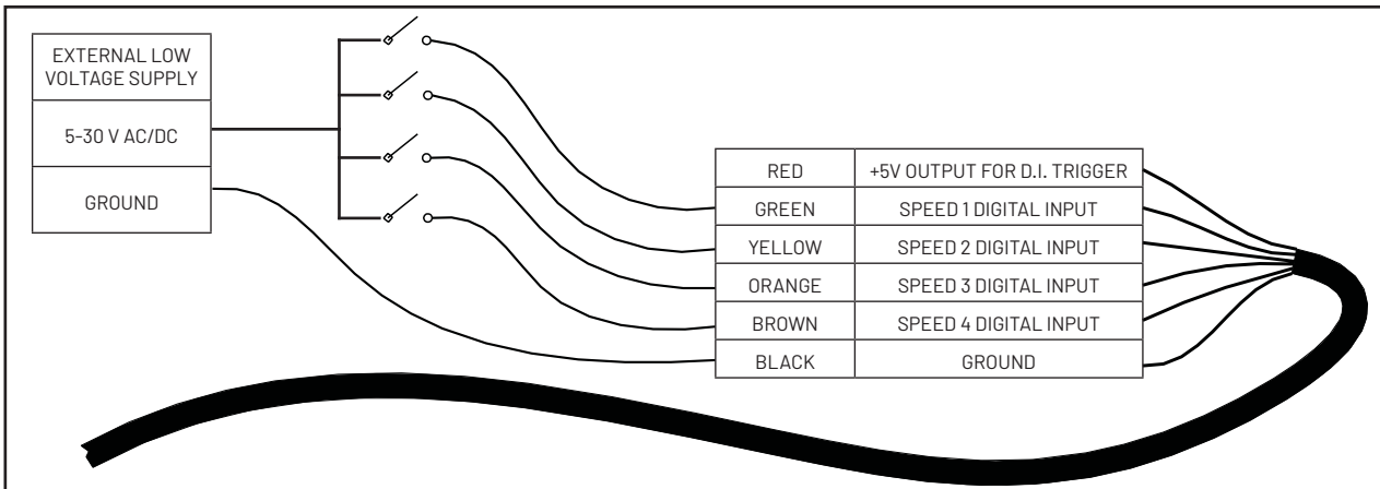
Figure 11: Low Voltage Power Supply Wiring Diagram
