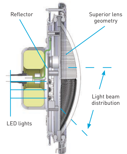
Drawing shows lens and reflector design which combine to provide superior light beam distribution.
